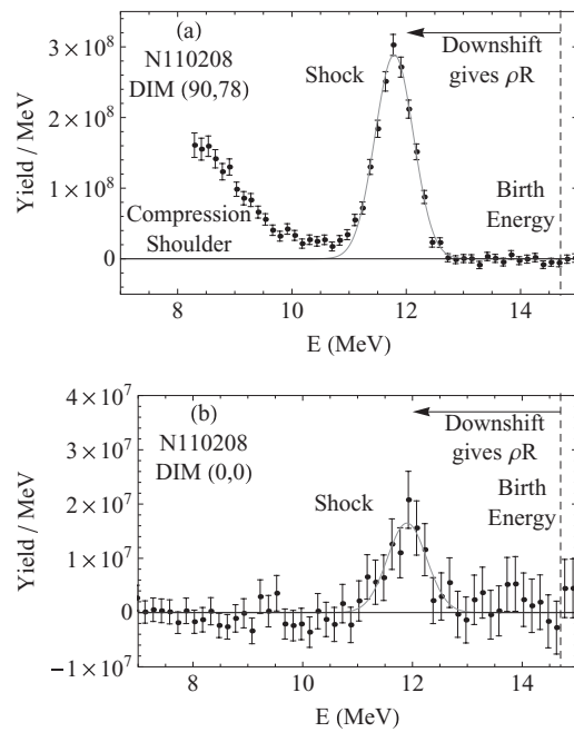
FIG. 3. D^3He proton spectrum measured on NIF shot N110208 (1.3 MJ shape tuning shot with a 544 Au hohlraum) on DIM (90,78) (a) and DIM (0,0) (b). The downshift from the birth energy at 14.7 MeV (dashed line) gives the \rho R . Gaussian fits to the shock peak are shown in gray. On the equator, Y_p = (2.43 \pm 0.44) \times 10^8 and E = 11.79 \pm 0.14 MeV, corrected for the hohlraum downshift, corresponding to \rho R = 68 \pm 8 mg/cm 2 . On the pole, we measured a yield of Y_p = (1.48 \pm 0.35) \times 10^7 and E = 11.90 \pm 0.26 MeV corresponding to \rho R = 65 \pm 10 mg/cm 2 .
