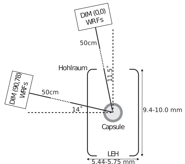
FIG. 2. Schematic of the experimental setup at NIF. The hohlraum is shown with capsule inside. The DIM (0,0) WRFs view the implosion through the laser entrance hole (LEH) at an angle of 11.5^\circ to the hohlraum axis, while the DIM (90,78) WRFs view through the hohlraum wall at an angle of 14^\circ to the equator.
