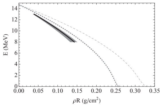
FIG. 1. D^3\text{He} proton energy versus total \rho R , calculated using the Li-Petrasso 22 dE/dx for various \rho R models: in a carbon-hydrogen (CH) plasma for the compression phase (dashed gray) and the shock phase (dotted gray). The black curve represents a HYDRA-derived model with error bars represented by the gray shaded region.
